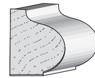
EC 172 Base Mould 9/16" x 3/4"
