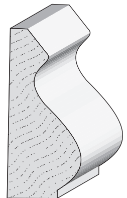
8456 Base Mould 3/4" x 1-3/4"
