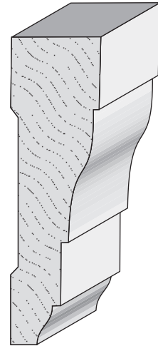
366 Casing 11/16" x 2-1/4"
