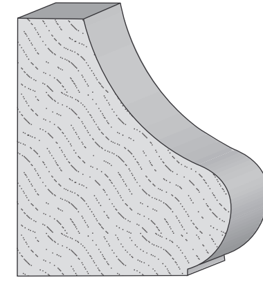
8048 Dilworth Brick Mould 1-3/4" x 2"
