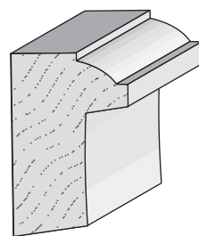
281 Backband 5/8" x 1"
