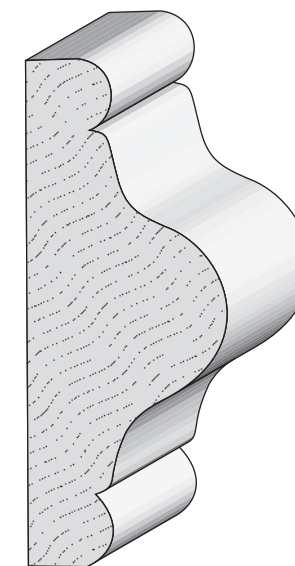
302 Chair Rail 1-1/16" x 2-3/4"
