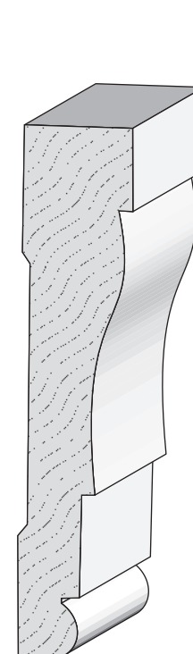
445 Casing 11/16" x 3-1/4"
