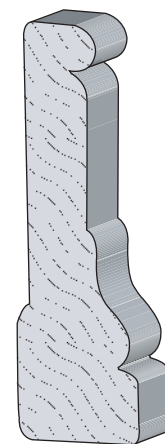
Cotswald Casing 3/4" x 2-1/4"
