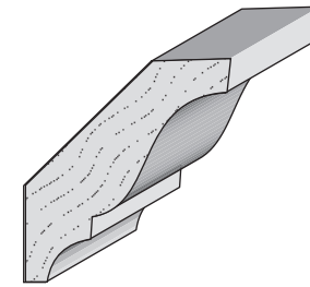
WP 68 Crown 1/2" x 1-3/4"
