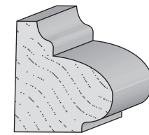
8620 Latta Base Mould 3/4" x 7/8"
