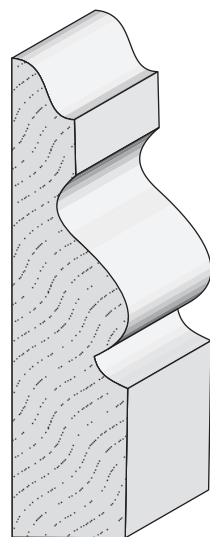
EC 212 Shingle Mould 11/16" x 2-1/2"
