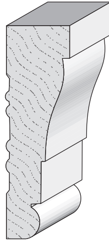
376 Casing 5/8" x 2-1/4"
