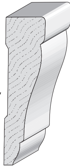
440 Casing 11/16" x 2-1/2"
