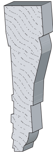
WM 361 Casing 11/16" x 2-1/2"
