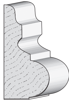
8174 Base Mould 3/4" x 1-5/8"
