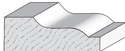
EC 210 Shingle Mould 9/16" x 1-5/8"
