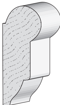
EC 273 5/8 x 1 3/4 Picture Mould
