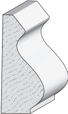
8456 Base Mould 3/4 x 1 3/4
