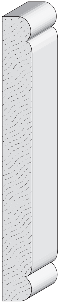
Chair Rail Backer 1/2 x 5 1/4
