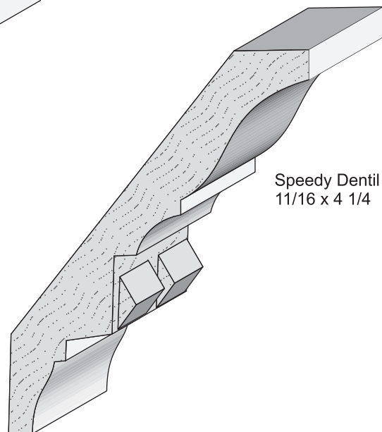
Curtis Crown 9/16 x 5
