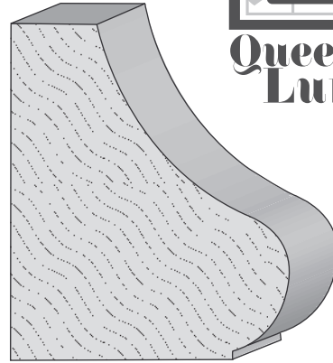
Dilworth Brick Mould 8048 1 3/4 x 2
