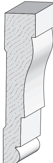
445 Casing 11/16" x 3-1/4"
