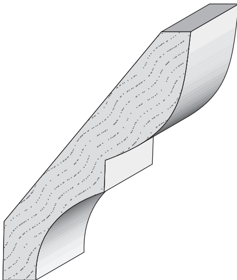
70 Bed Mould 9/16" x 2-3/4"
