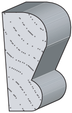
Beauty Mould 5/16" x 11/16"
