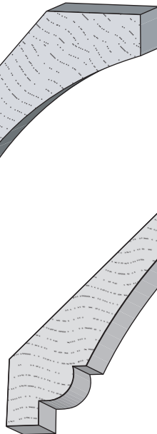
EC 50, CROWN 11/16" X 5-1/4"
