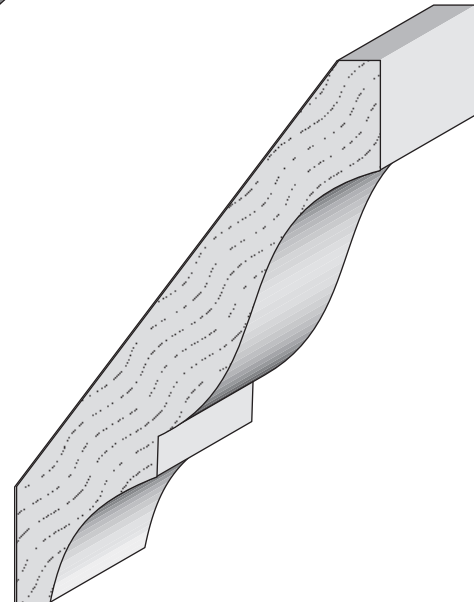
WP 51 Crown 9/16" x 3-1/4"
