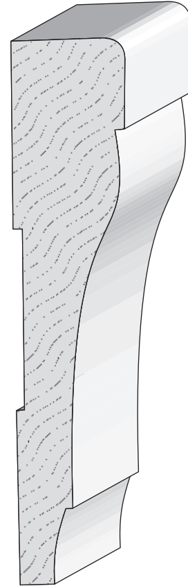
Like 440 Casing 3/4" x 3-9/16"
