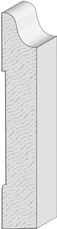
8384 Old Style Base 3/4" x 4-1/2"
