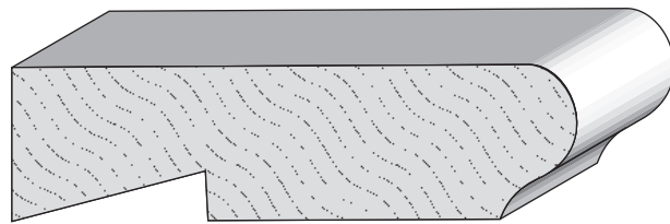
WM 1163 - A 7/8" Cutout Stool 1" x 3-1/4"
