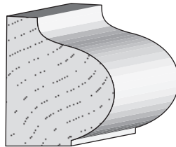
WM 172 Base Mould 9/16" x 3/4"
