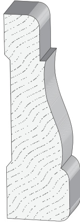
WM356 Casing 11/16" x 2-1/4"
