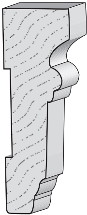
Wilmore Casing 3/4" x 2 1/4"
