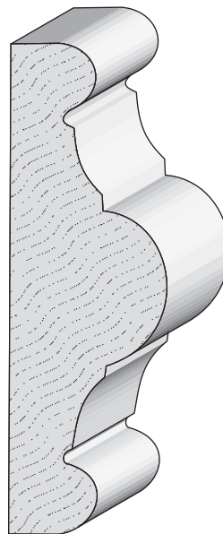
Hatley Chair Rail 1-1/8" x 3-1/2"
