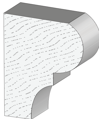
Eastover Solid Bed Mould 1-5/8" x 2"
