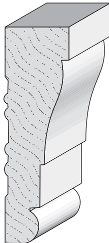
376 Casing 5/8" x 2-1/4"
