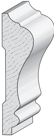
WM 390 Chair Rail 11/16" x 2-5/8"
