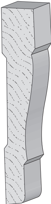
444 A Casing 11/16" x 3-1/2"
