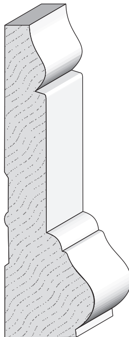
460 Casing 1" x 3-5/8"
