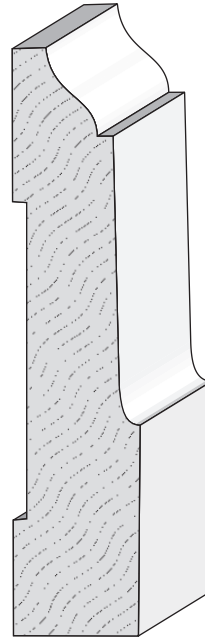
8711 Dilworth Casing 3/4" x 3-1/2"
