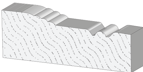
Presidential Brick Mould 1-1/4" x 3-1/2"
