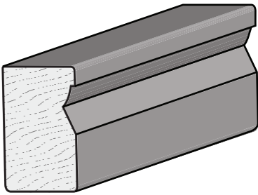
Kolbe Brick Mould 1" x 2"
