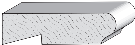
WM 1195 Stool 11/16" x 2-1/2"
